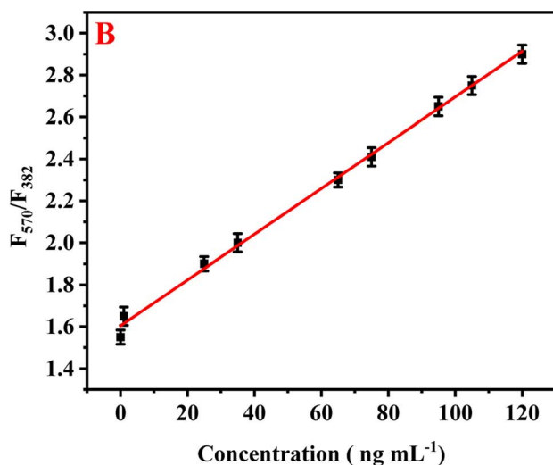
Fig. 3 (A) The effect of different concentrations of vancomycin (0.0–120.0 ng mL -1 ) on the fluorescence intensity of Co@DECDS system. (B) Relationship of ( F_{570}/F_{382} ) versus vancomycin concentrations.
