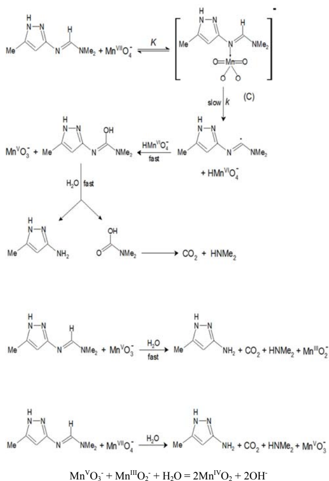
Scheme 1. Mechanism of oxidation of methylaminopyrazole formamide by permanganate ion in neutral medium.
