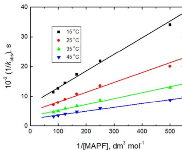
Figure 4. Plots of 1/k_{\text{obs}} versus 1/[\text{MAPF}] in the oxidation of methylaminopyrazole formamide by permanganate ion in neutral medium at different temperatures. [\text{MnO}_4^-] = 4.0 \times 10^{-4} \text{ mol dm}^{-3} .
