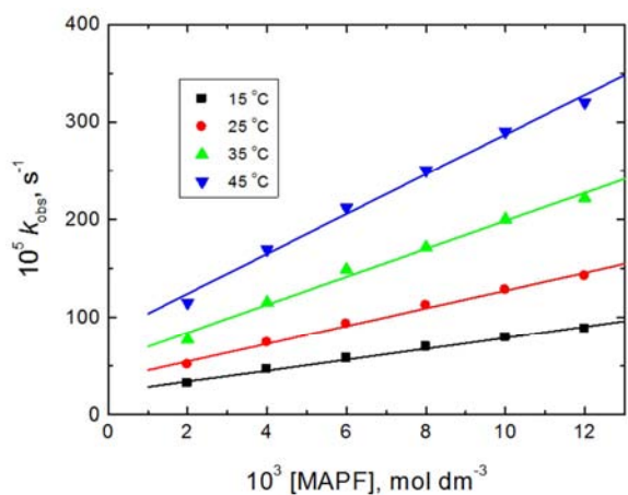
Figure 2. Plots of the observed-first order rate constants ( k_{\text{obs}} ) versus MAPF concentration in the oxidation of methylaminopyrazole formamide by permanganate ion in neutral medium at different temperatures.
