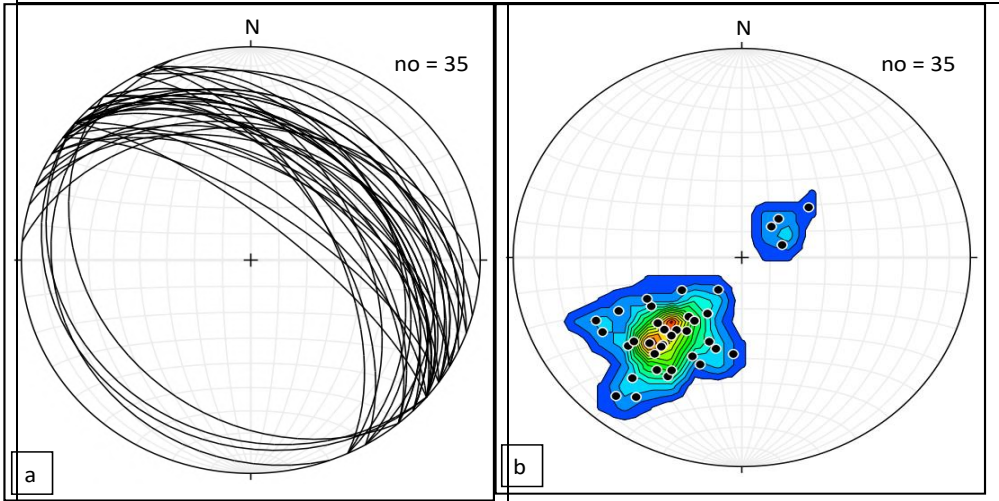
Fig. 8: Foliation planes (a) and their poles contouring (b) related to D_3 deformation phase.
